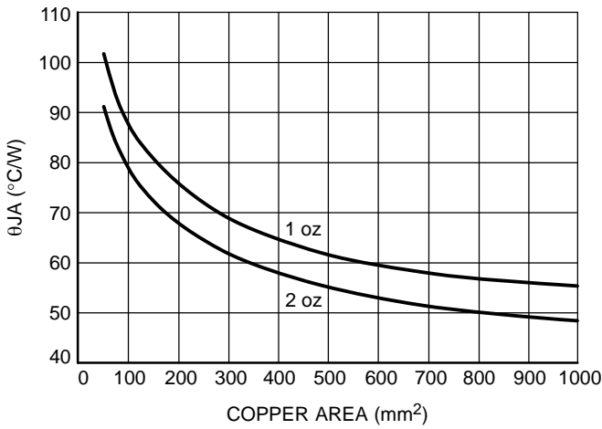
Figure 8. \theta_{JA} vs. Copper Spreader Area
